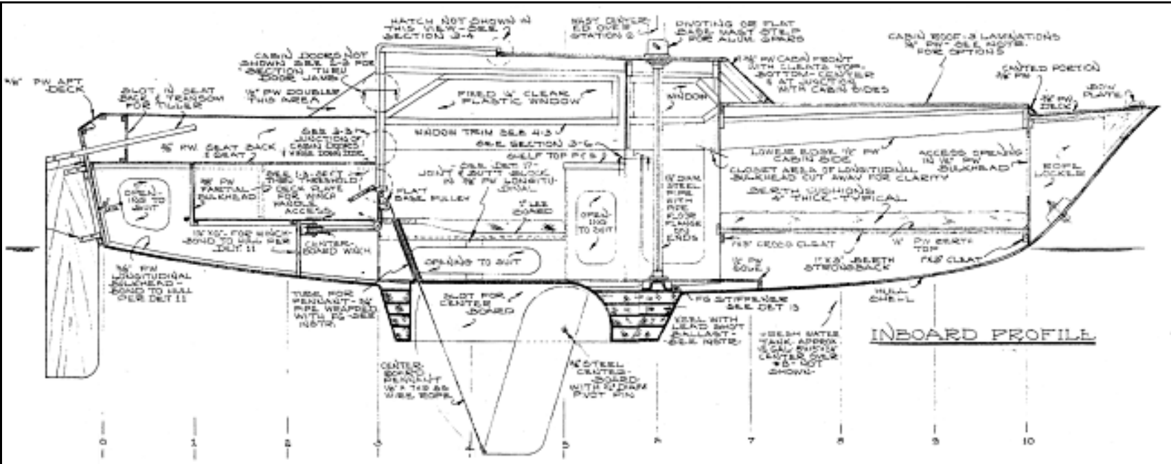
GLEN-L 6.9 Inboard Profile
