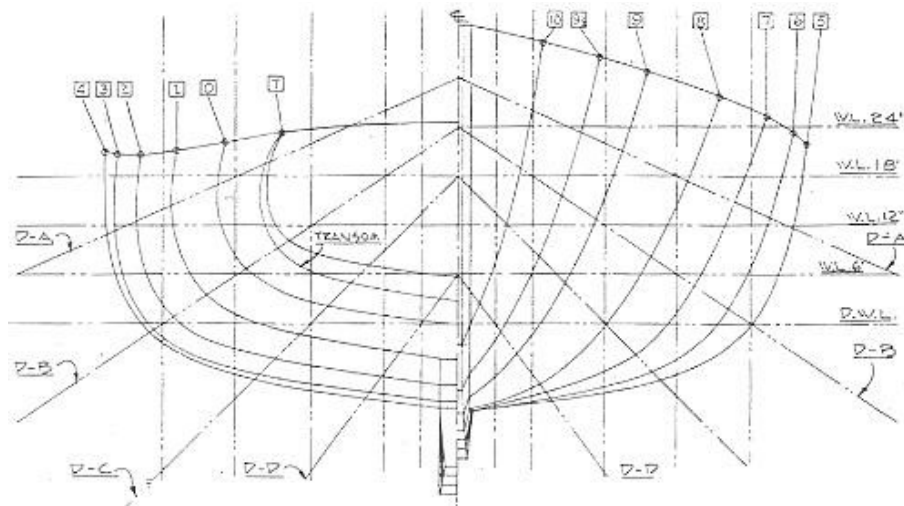
Harbor Master Body Plan
