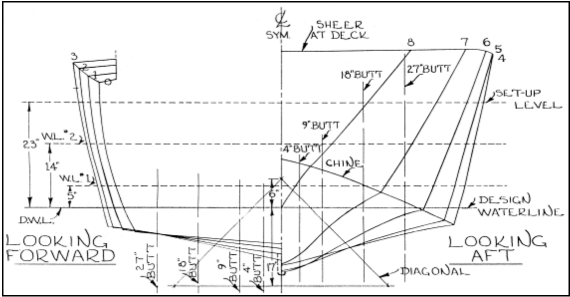
Sections drawing
